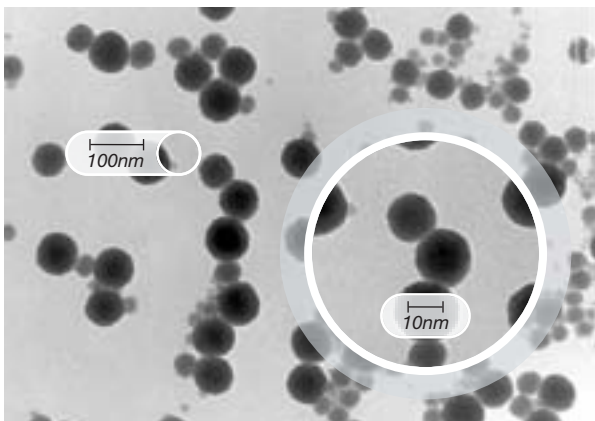
TEM picture of polydisperse LUDOX® colloidal silica
